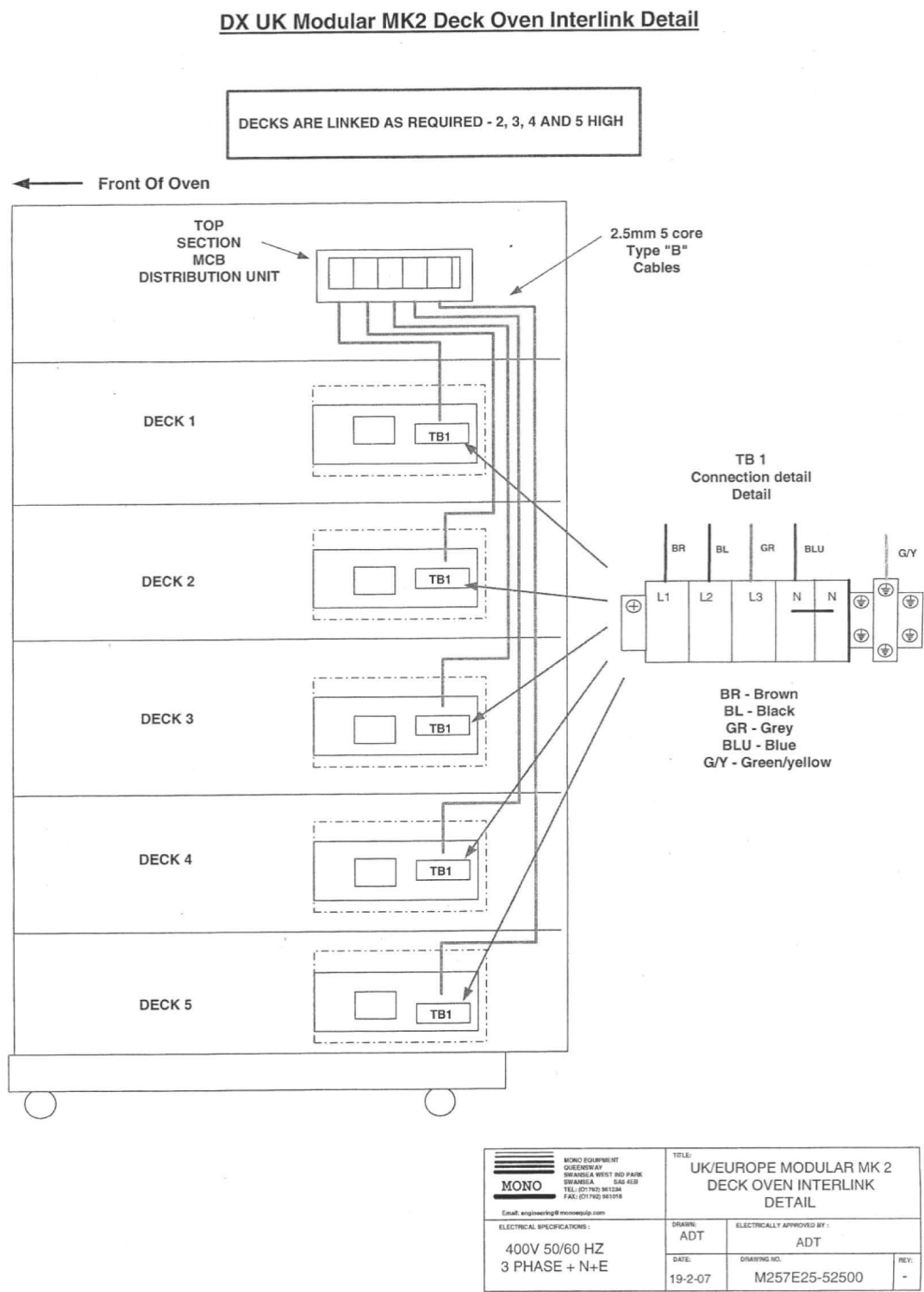
Figure D.2: Modular Mk2 deck oven interlink detail drawing M257E25-52350
