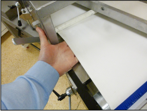
Upper Belt Tensioning
